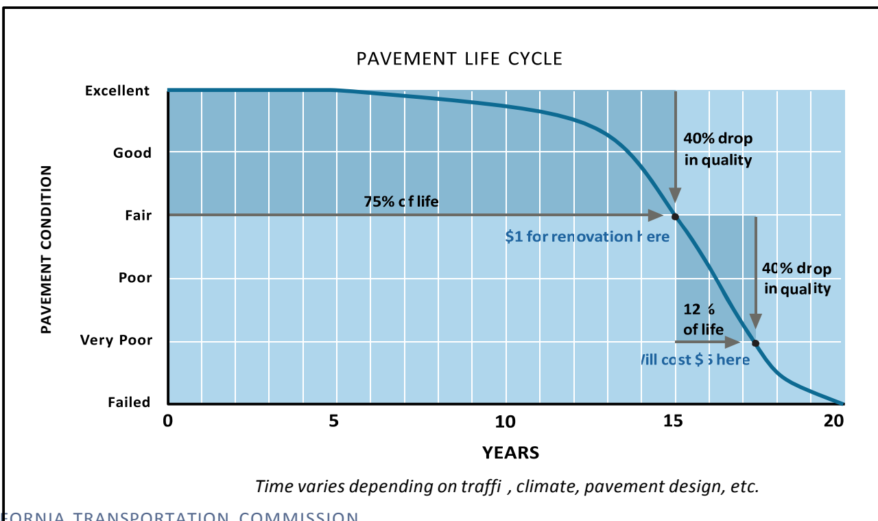
Figure 7 -Pavement Life Cycle Chart
