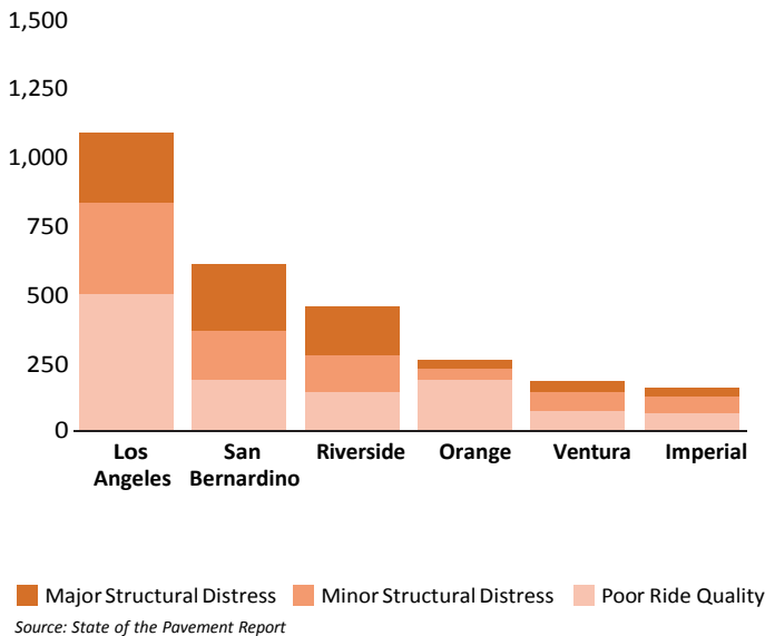
FIGURE 8 – Southern California Total State Highway System Distressed Lanes Miles by County (2013)
