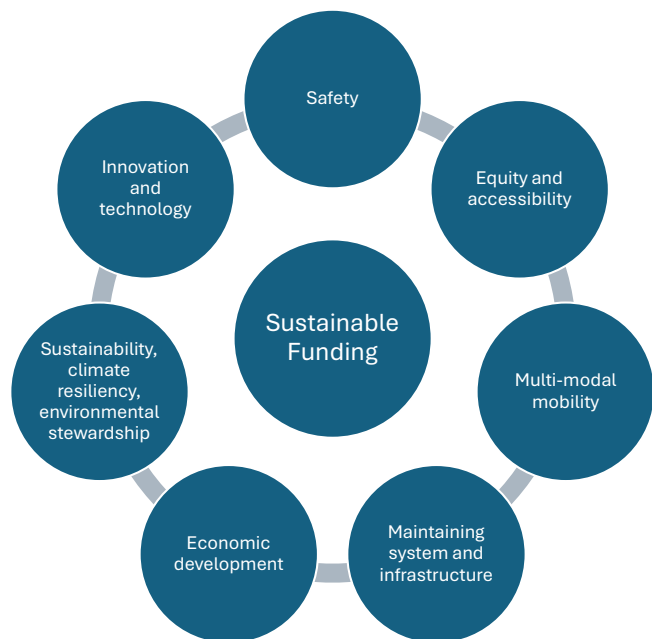
Figure 2. First principles.
