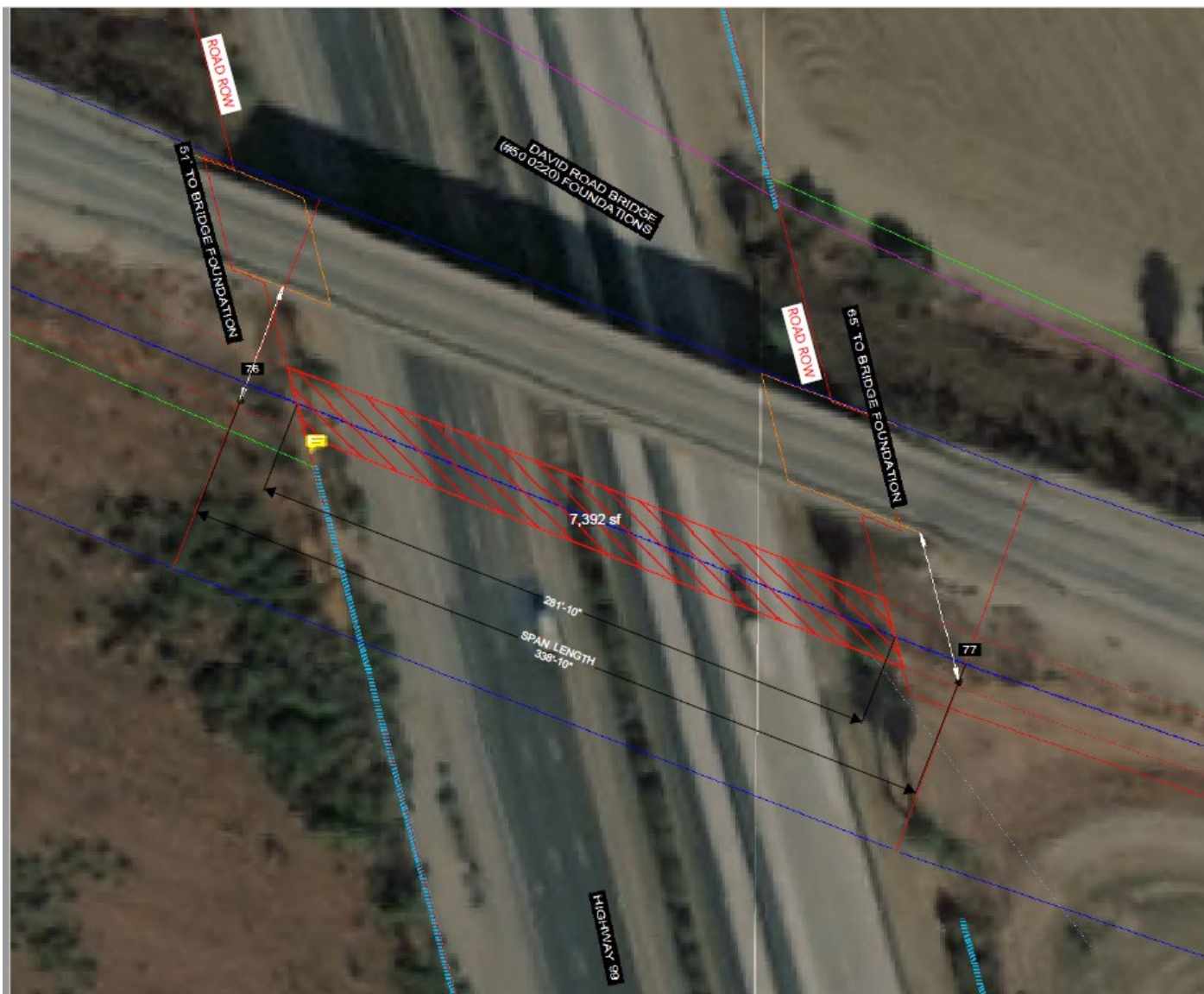
Approximate Dimensions that Proposed Aerial Transmission Lines Will Span
